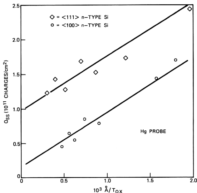
Fig. 15—Plot of Q_{ss} after \text{Al}_2\text{O}_3 deposition as a function of the \text{SiO}_2 thickness for n -type, \langle 100 \rangle and \langle 111 \rangle , Si substrates.
