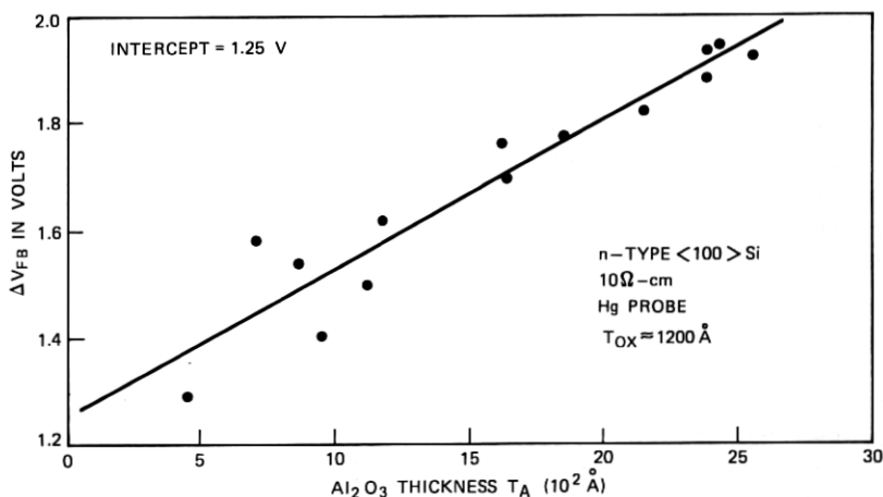
Fig. 9—Plot of the corrected differential flatband voltage as a function of the \text{Al}_2\text{O}_3 thickness for a constant \text{SiO}_2 thickness ( T_{ox} = 1200 \text{ Å} ) on n -type, \langle 100 \rangle , Si substrates.
