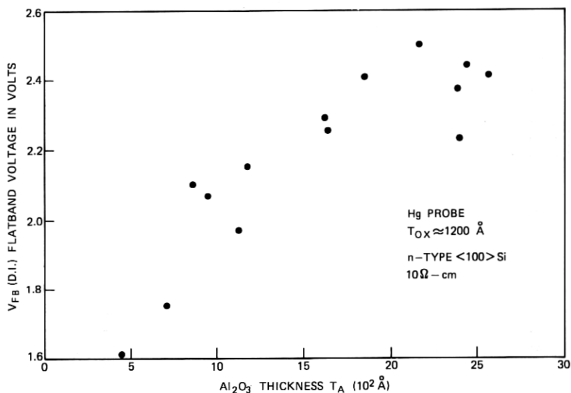
Fig. 8—Plot of the Hg/ \text{Al}_2\text{O}_3 / \text{SiO}_2 /Si flatband voltage as a function of the \text{Al}_2\text{O}_3 thickness for a constant \text{SiO}_2 thickness ( T_{ox} = 1200 \text{ Å} ) on n -type, \langle 100 \rangle , Si substrates.
