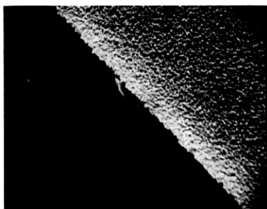
5 MIN ETCH-BACK T_A \approx 1250 Å
